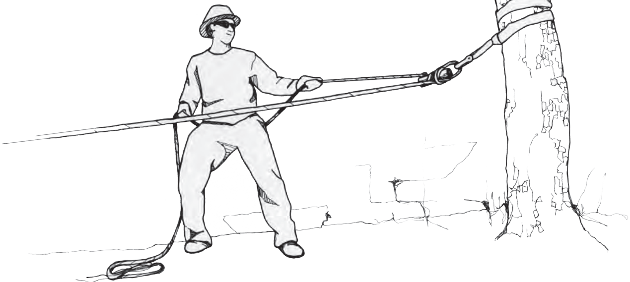
Figure 14–2—A friction braking belay system used for light loads in various aerial rigging configurations.
