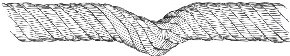
Figure 2-9—Kinking (caused by a loop in wire rope under tension).
