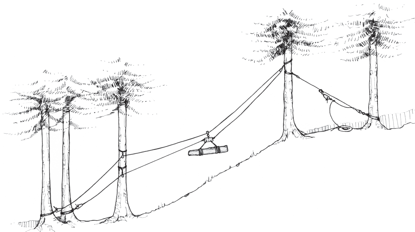
Figure 13–10—A typical running-skyline configuration using a tail block and carriage (note the use of a spar tree back guy).
