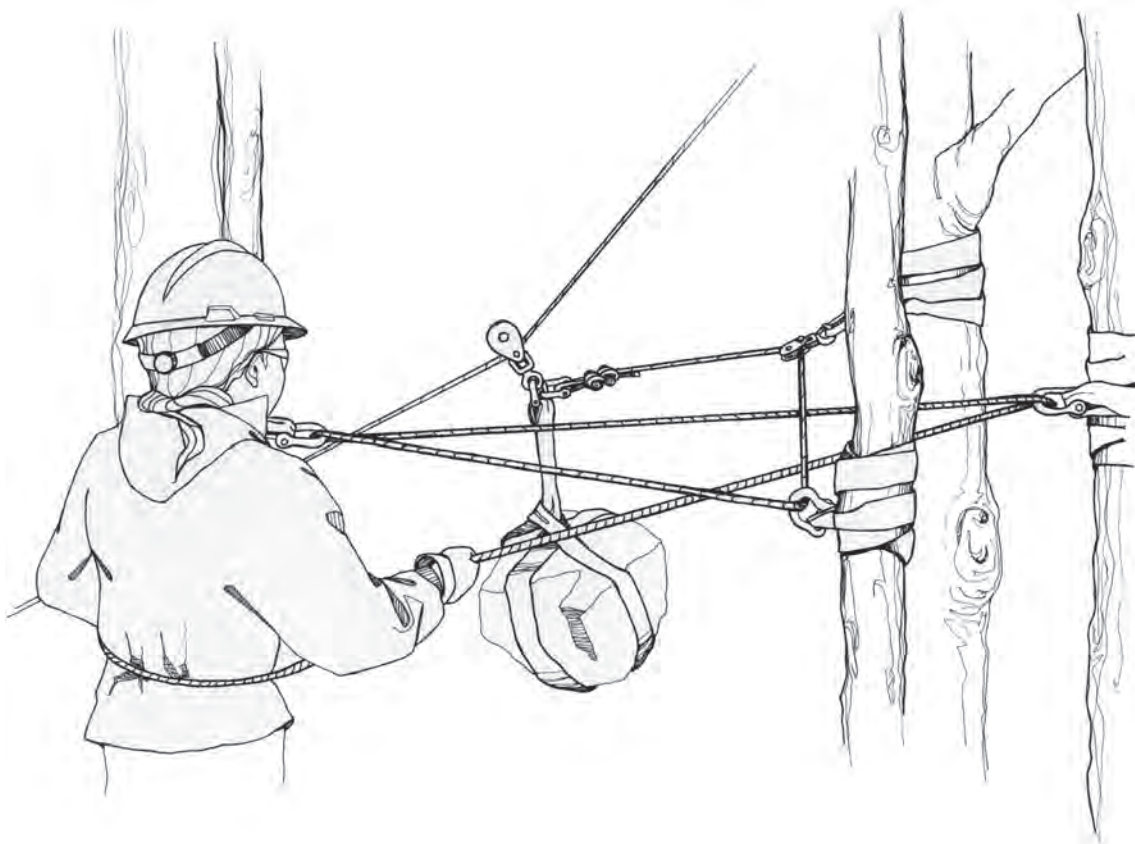
Figure 14-1 — A three-point friction belay and directional block.
