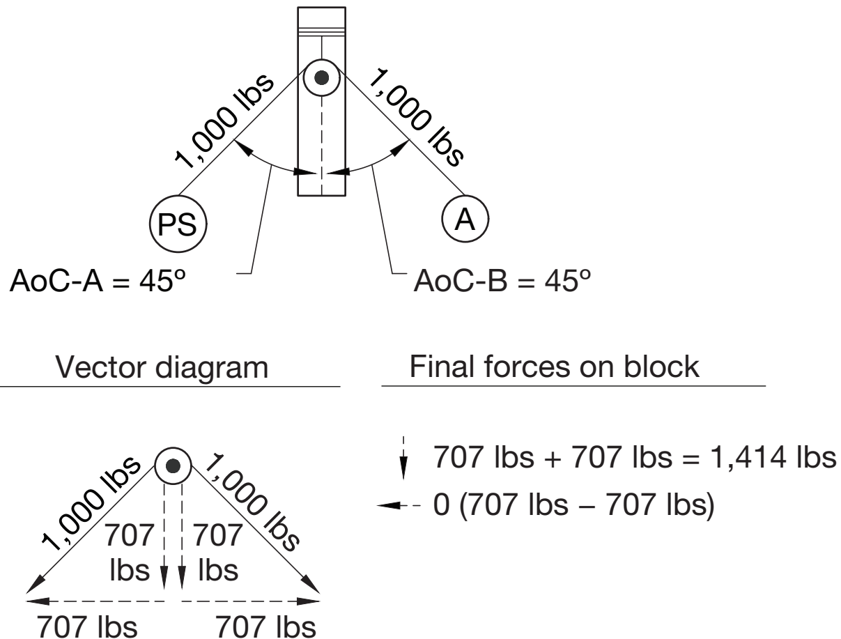
Figure D-10—Vertical and horizontal forces when lines enter and leave a block at the same angle.
