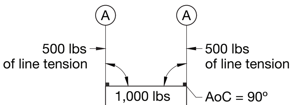
Figure E-4 – The line tension with two suspending lines equals half the load weight in each line.
