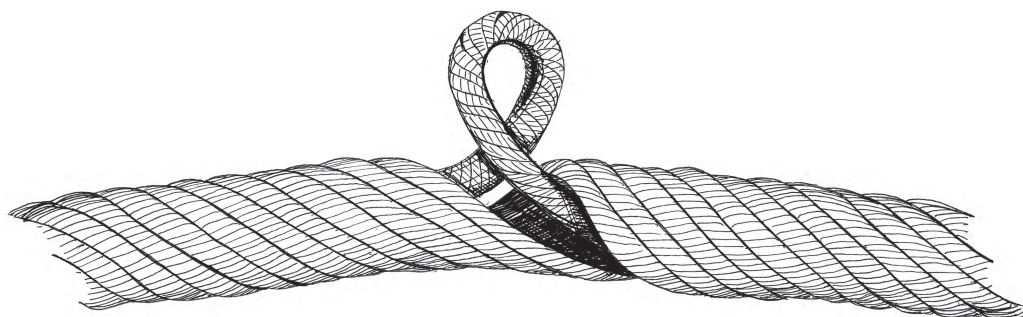
Figure 2–11—A popped core or core protrusion (usually caused in wire rope by rotation, the sudden release of a load, or core slippage).
