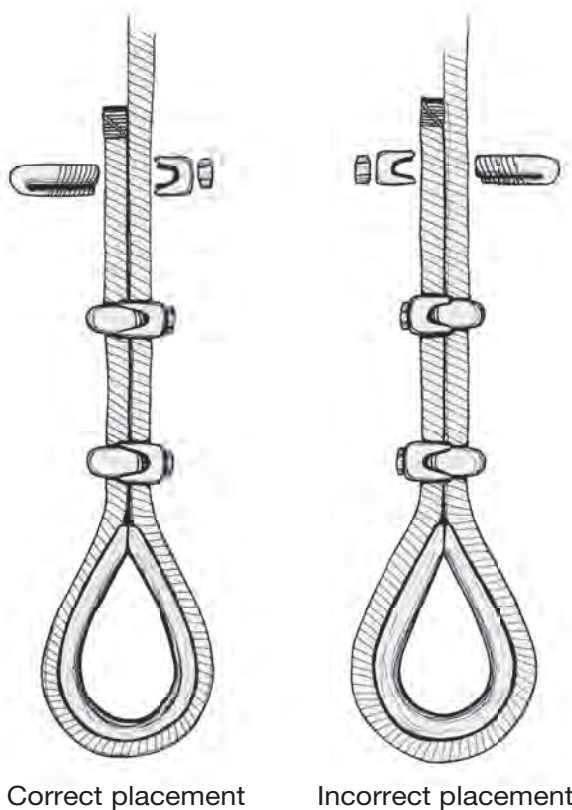
Figure 7–12 — The correct and incorrect placement of wire rope clips.
